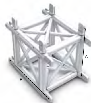
3 WAY T-PIECE VERTICAL
