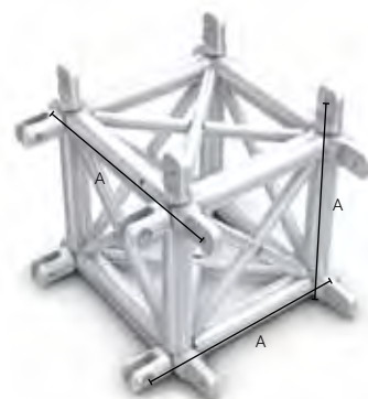
3 WAY CORNER 90° MALE DOWN
